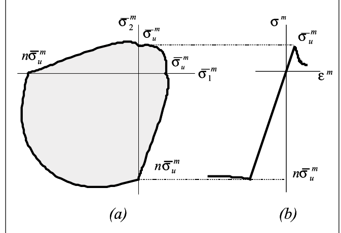
Figure 2 - Damage model: (a) damage criterion in the effective stress space, (b) one-dimensional stress-strain curve
