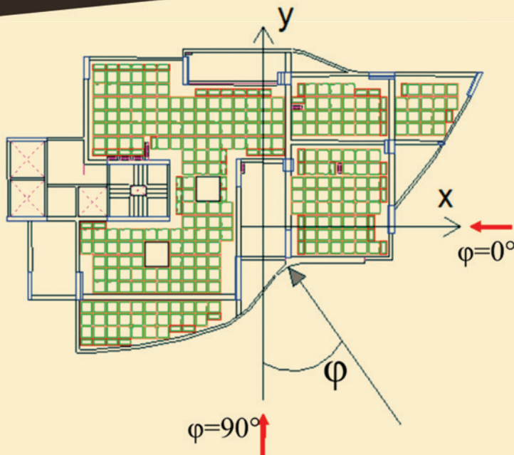
(a) Floor plan and wind incidence angle \phi
