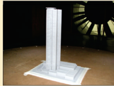
(b) Wind tunnel test model
